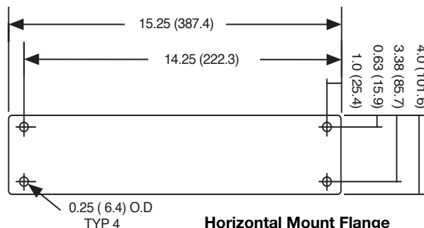
HM Configuration Side View
