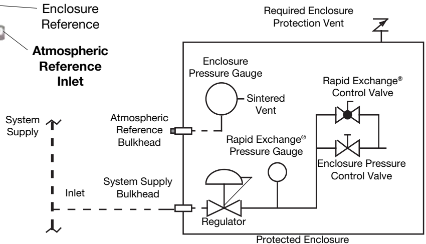
Model 3003-LPS-CI-Z-VM Shown w/ GCK installed
