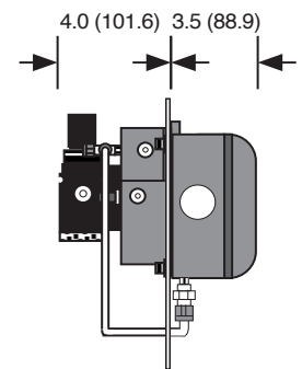
HM Configuration Side View
