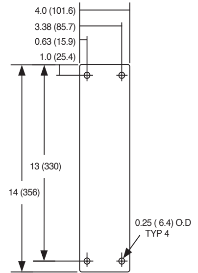
Vertical Mount Flange Front View
