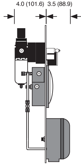
VM Configuration Side View
