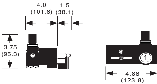
Side View Pneumatic Manifold
