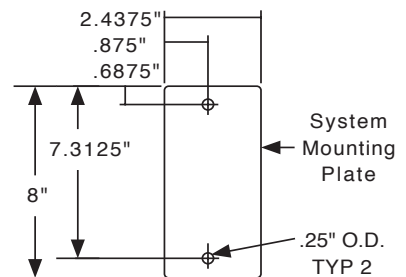
Universal Mounting Bracket
