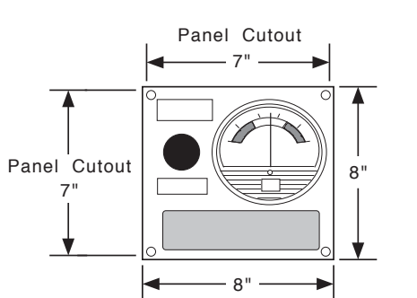
1011-FM & 1011-PM (Frame & Panel Mount Configuration)
